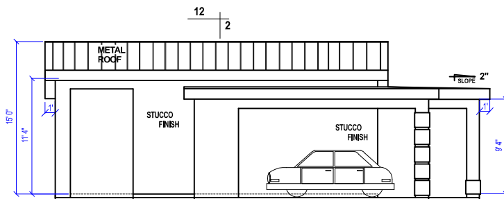
LEFT SIDE ELEVATION SCALE=1/4"=1'-0"
