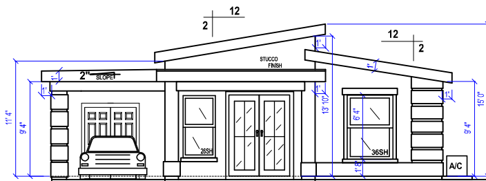
FRONT ELEVATION SCALE=1/4"=1'-0"
