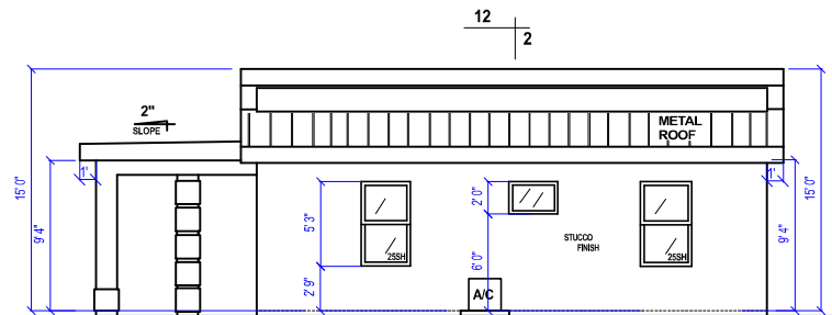
RIGHT SIDE ELEVATION SCALE=1/4"=1'-0"
