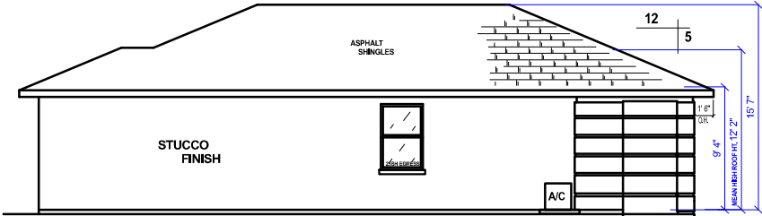
LEFT SIDE ELEVATION SCALE=1/4"=1'-0"
